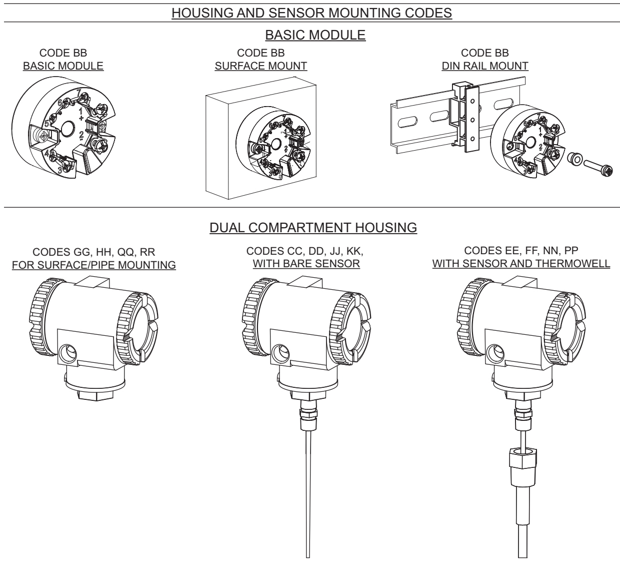
Figure 1. Available Housing and Sensor Mounting Codes
