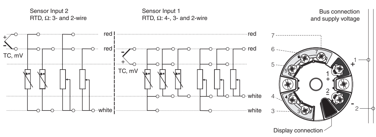
Figure 2. Input Connections – Basic Transmitter
