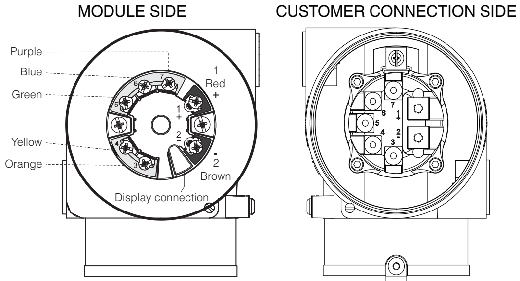
Figure 3. Dual Compartment Housing Wiring from the Terminal Block to the Module
